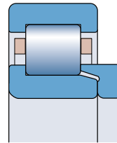
NJ design + HJ angle ring
